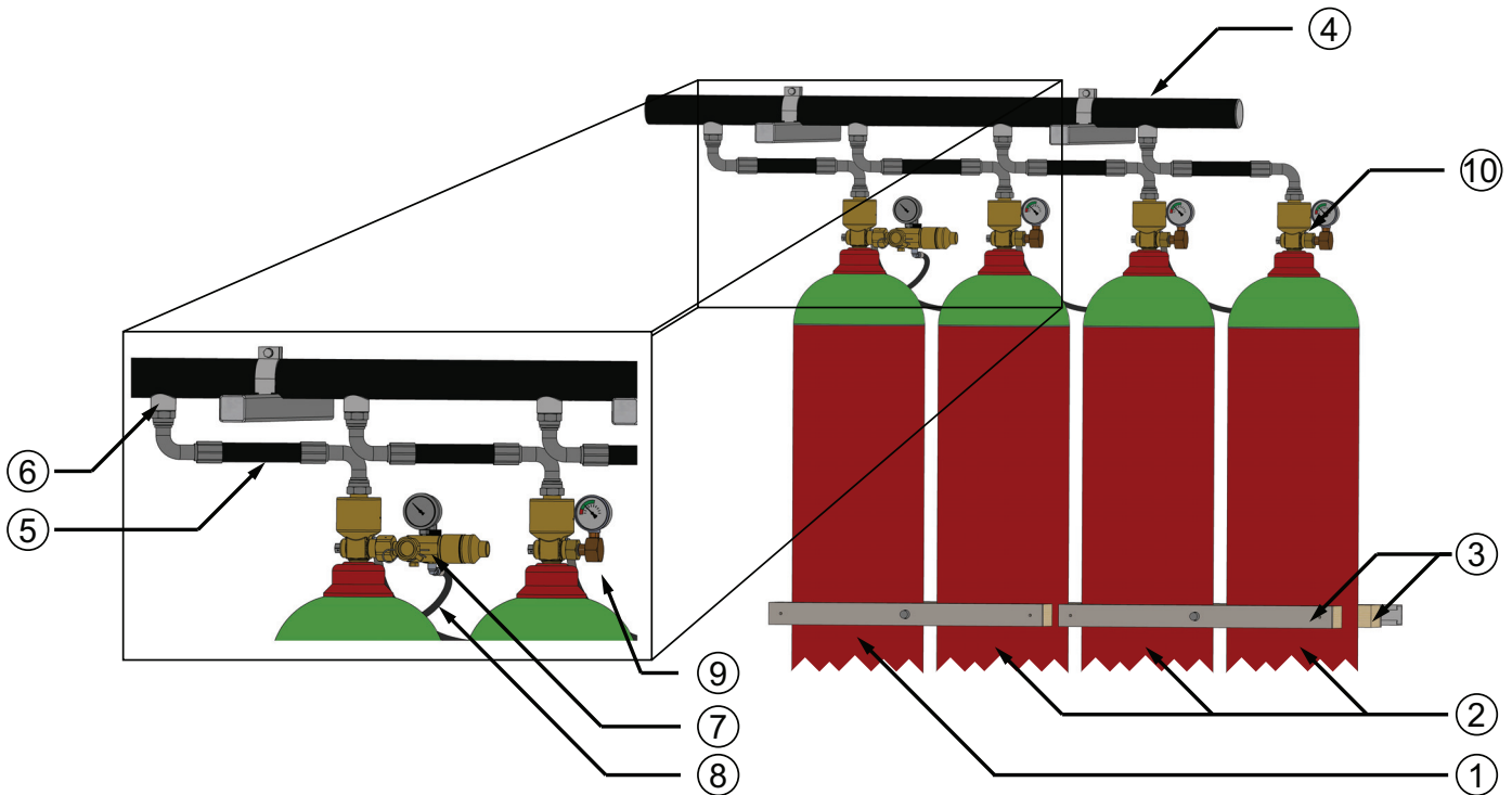
Figure 1. Single Area Cylinder Bank Arrangement
