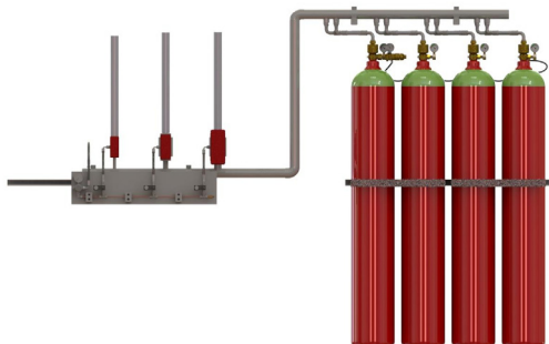
Figure 13. Selector Valve Setup
